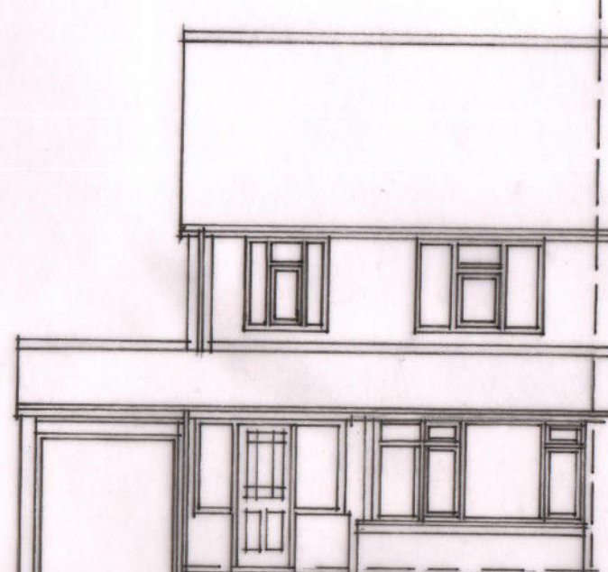
FRONT ELEVATION (EXISTING) 1:100
