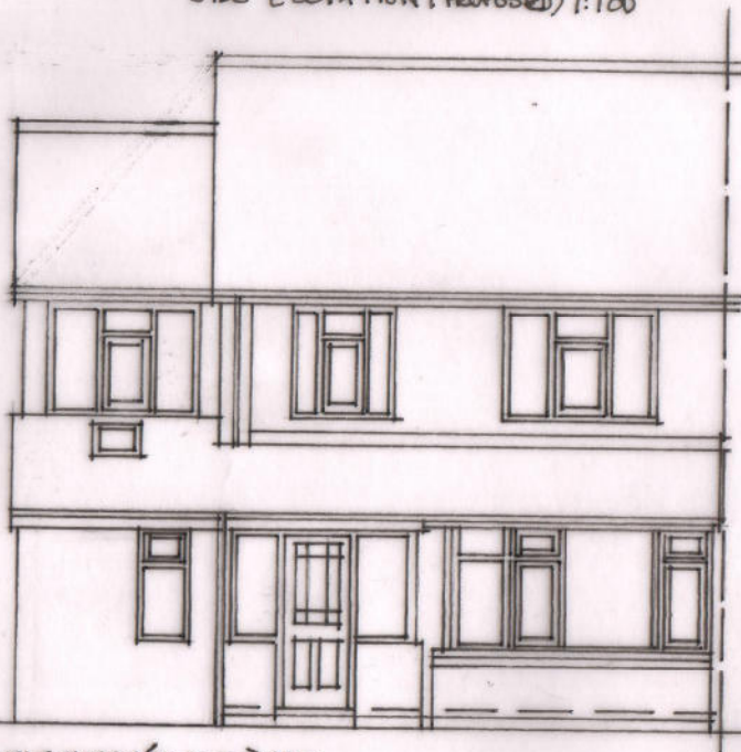
FRONT ELEVATION (PROPOSED) 1:100
